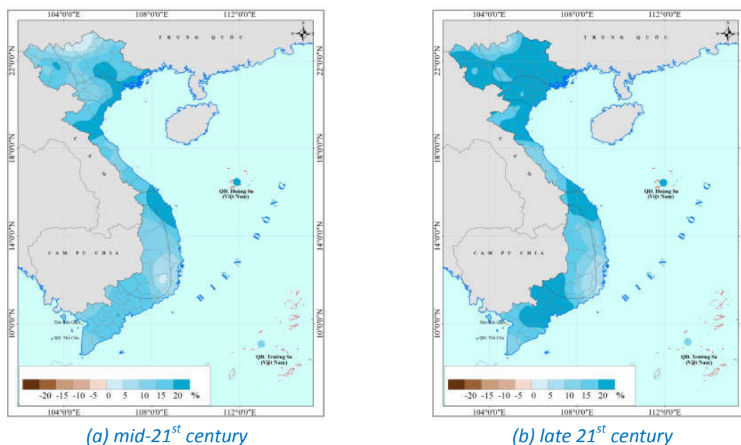
Figure 16. Changes in annual rainfall (%) based on RCP8.5 scenarios
