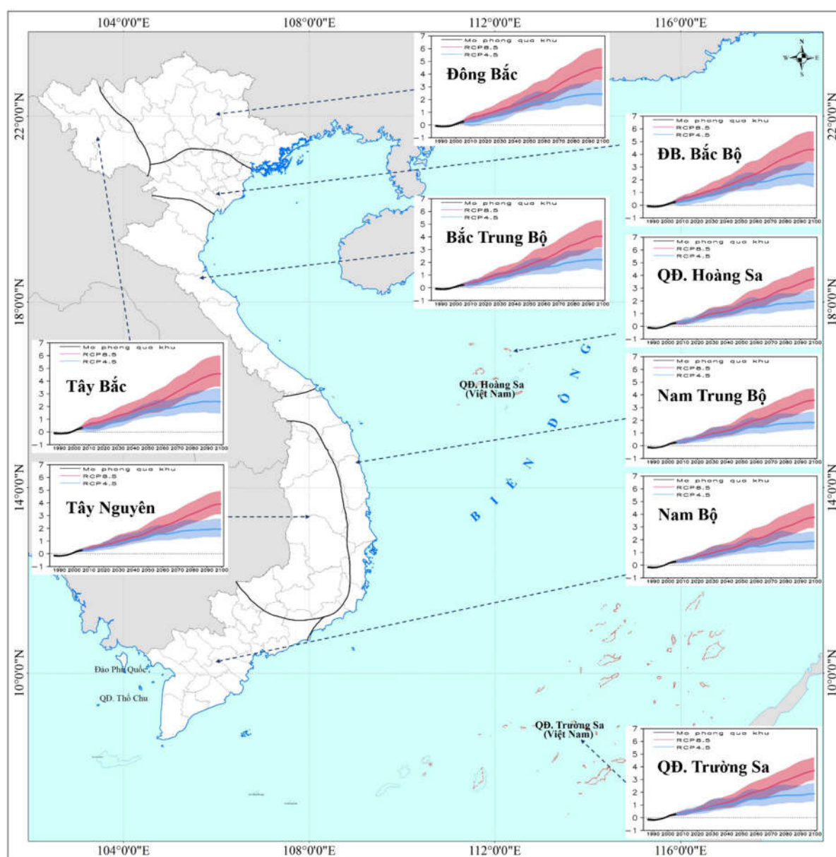
Figure 10. Changes in average annual temperature (°C) over 7 regions and islands of Viet Nam
