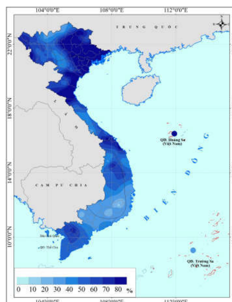
b) Based on RCP8.5 scenarios
