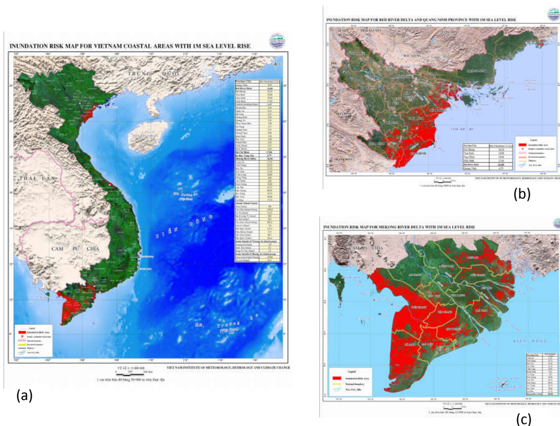
Figure 20. Inundation maps with a sea level rise of 100 cm
