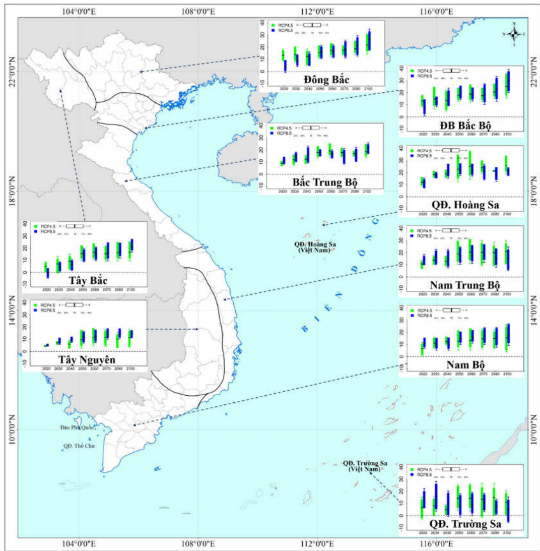
Figure 14. Changes in annual rainfall (%) over 7 regions and islands of Viet Nam
