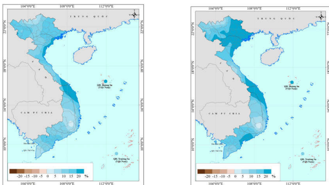
Figure 15. Changes in annual rainfall (%) based on RCP4.5 scenarios
