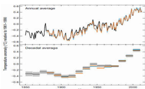
Figure 1. Temperature deviation (1850-2012) compared to the period 1961-1990 (IPCC, 2013)
