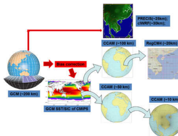
Figure 9. Climate projections using dynamical downscaling procedures
