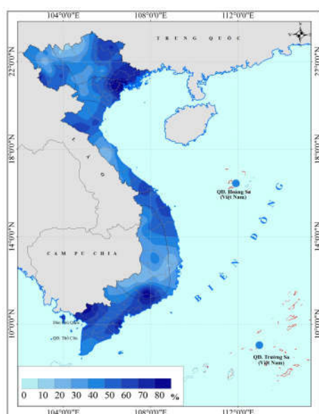
a) Based on RCP4.5 scenarios
