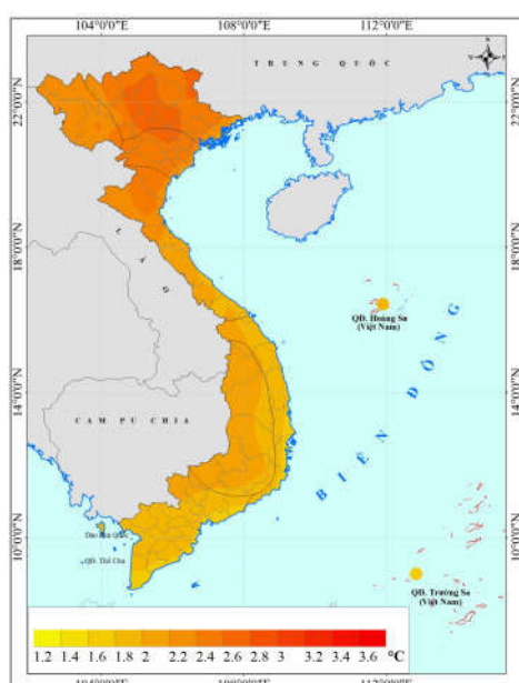
a) Average annual maximum temperature
