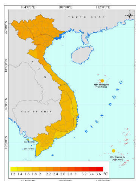
b) Average annual minimum temperature
