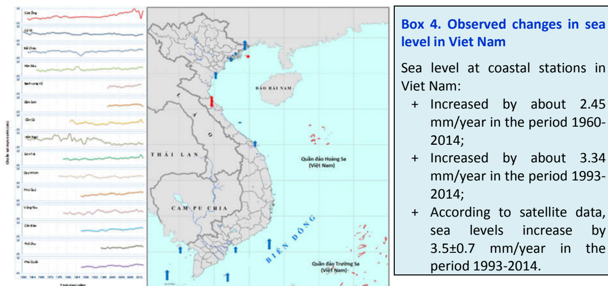
Figure 6. Changes in sea level
