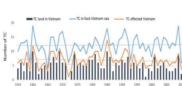
Figure 5. Evolution of typhoons and tropical depressions in the period 1959-2014
