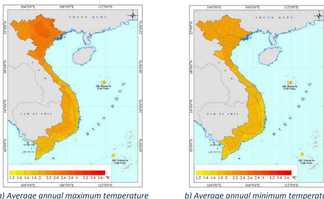
Figure 13. Changes in maximum and minimum temperatures (°C) by late 21 st century based on RCP4.5 scenarios
