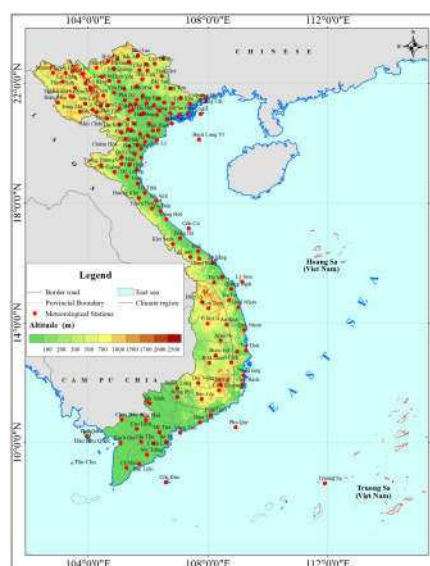
Figure 7. Meteorological stations
