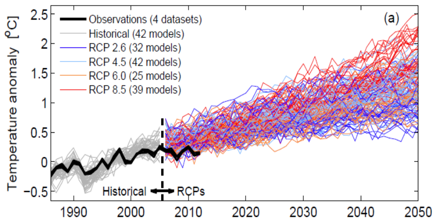
Global mean temperature near-term projections relative to 1986–2005
